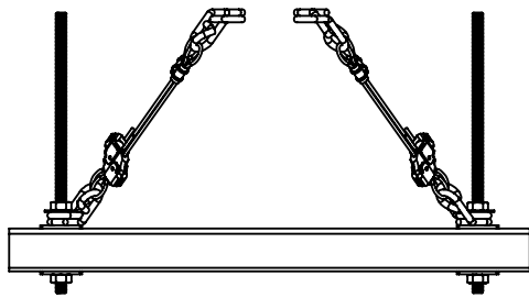
SECTION THRU TRAPEZE ALTERNATIVE CABLE TRANSVERSE BRACE PATTERN
