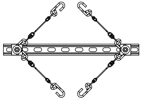
OVERHEAD VIEW ALTERNATIVE SPLOYED CABLE BRACE PATTERN
